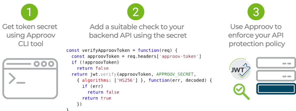
Figure 4. Integration into the backend API
