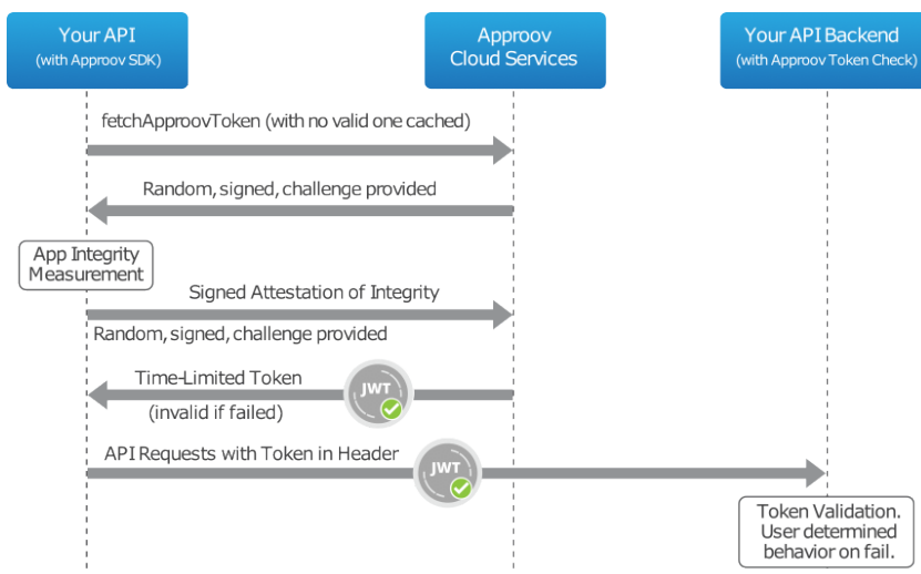
Figure 5. App authentication protocol
