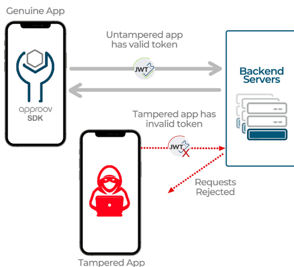
Figure 9. How Approov restricts accesses to legitimate apps only
