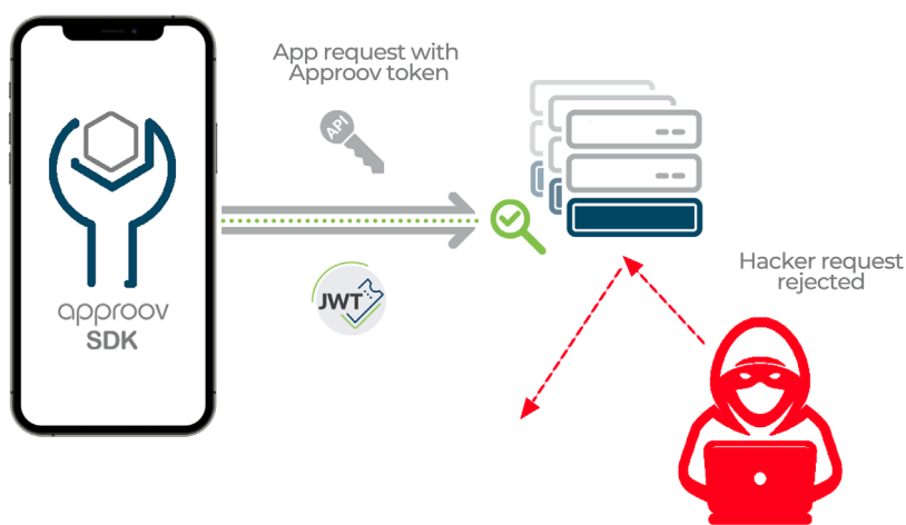
Figure 1. Approov Protects Digital Assets Exposed by APIs
