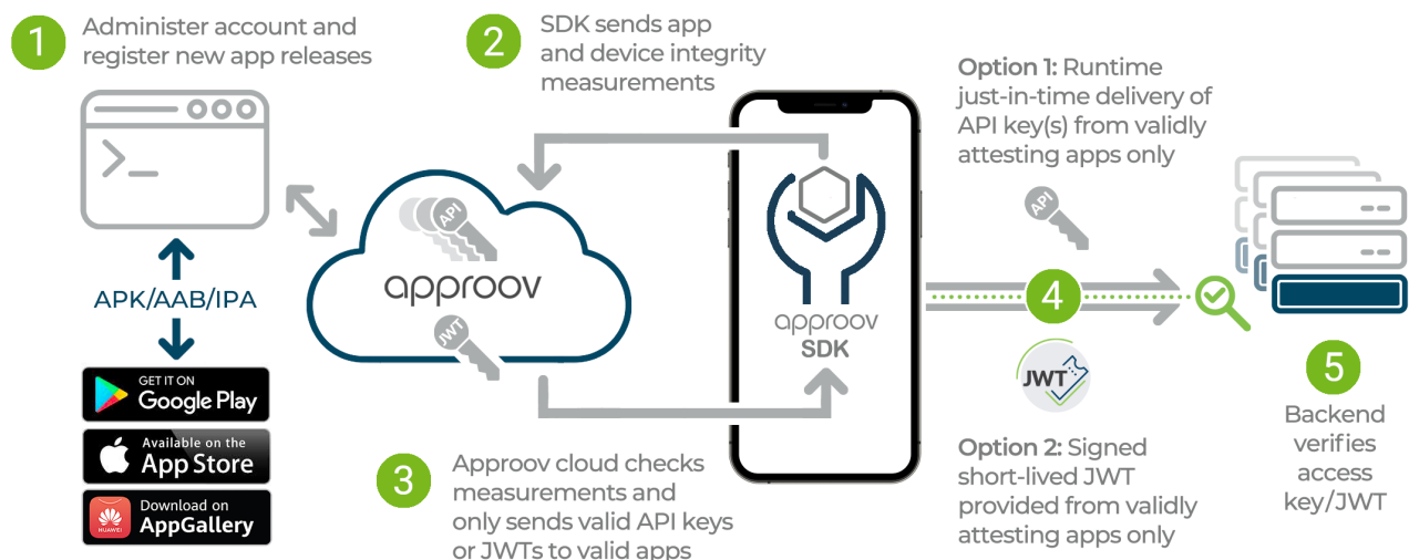
Figure 2. The Components of Approov
